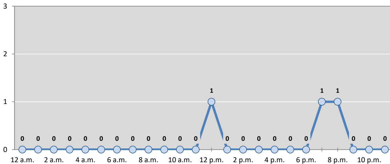
Figure 3: Alcohol-involved Crashes by Hour in Hatch, 2024
