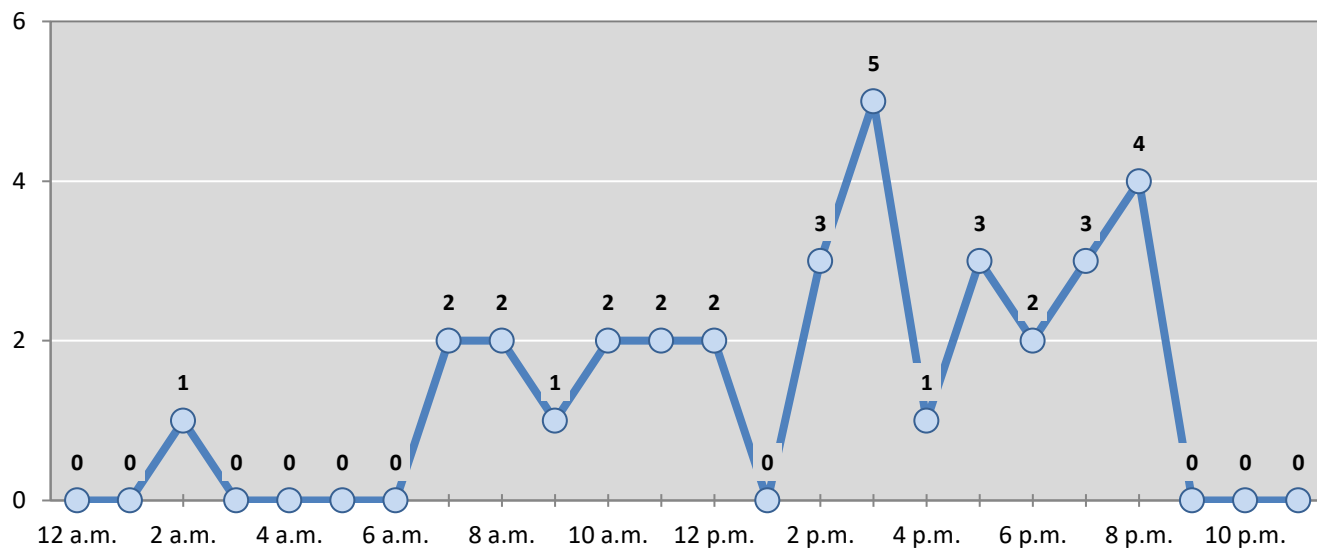
Figure 2: Crashes by Hour in Hatch, 2024
