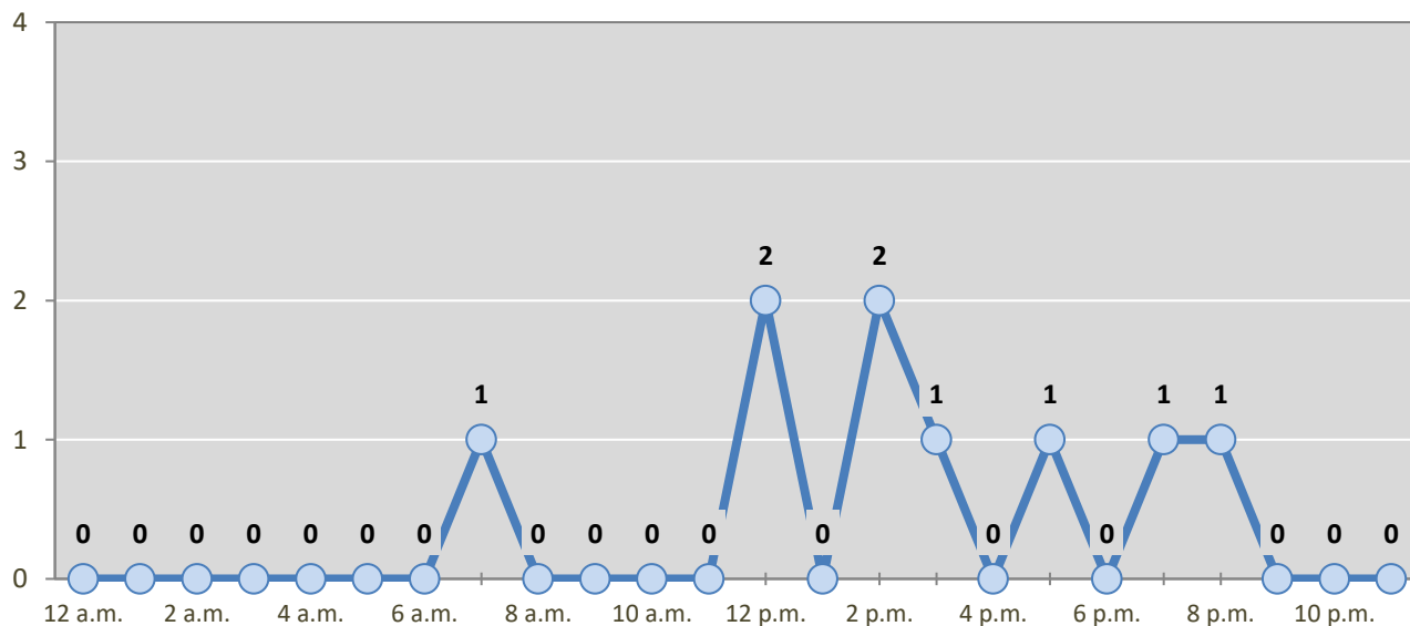
Figure 4: Fatal and Injury Crashes by Hour in Hatch, 2024
